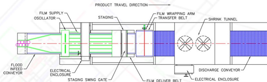
Flood Infeed
